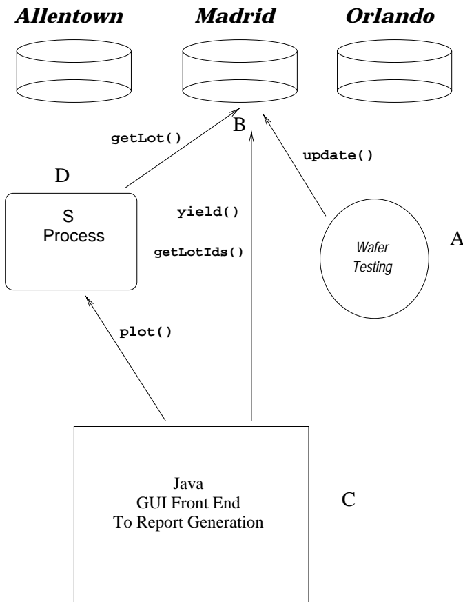
Figure 2: Viewing test results, with CORBA providing the interaction. Arrows indicate invocation of the corresponding method, pointing towards the server providing the method.
